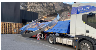
TRANSPORTING A FORGED RING: 5.80MT DIAMETER, 24 TONS
